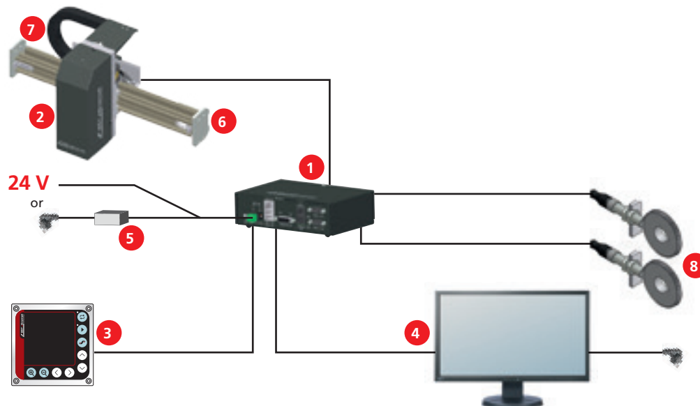
1 Controller 2 Camera 3 external operating panel (opt. touch monitor) 4 Monitor (opt. touch monitor) 5 Controller power supply 6 Traverse (opt. motorized) 7 Cable track 8 Synchronization
